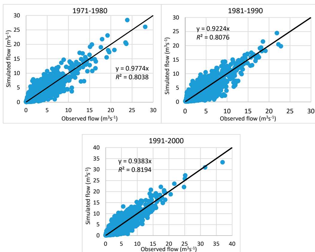
Figure 7. Relationship between the observed and simulated daily flow of the River Frome in Bristol.
